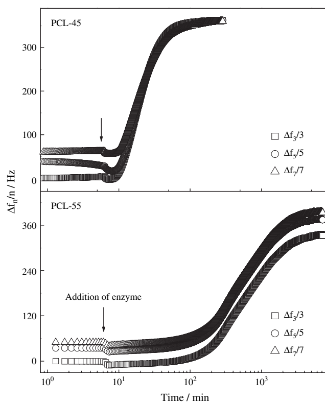
Fig. 2. The frequency shift ( \Delta f ) of QCM during enzymatic degradation of PCL-45 and PCL-55 catalyzed by lipase PS, where C_e = 0.5 mg/mL and n = 3, 5, 7 .
