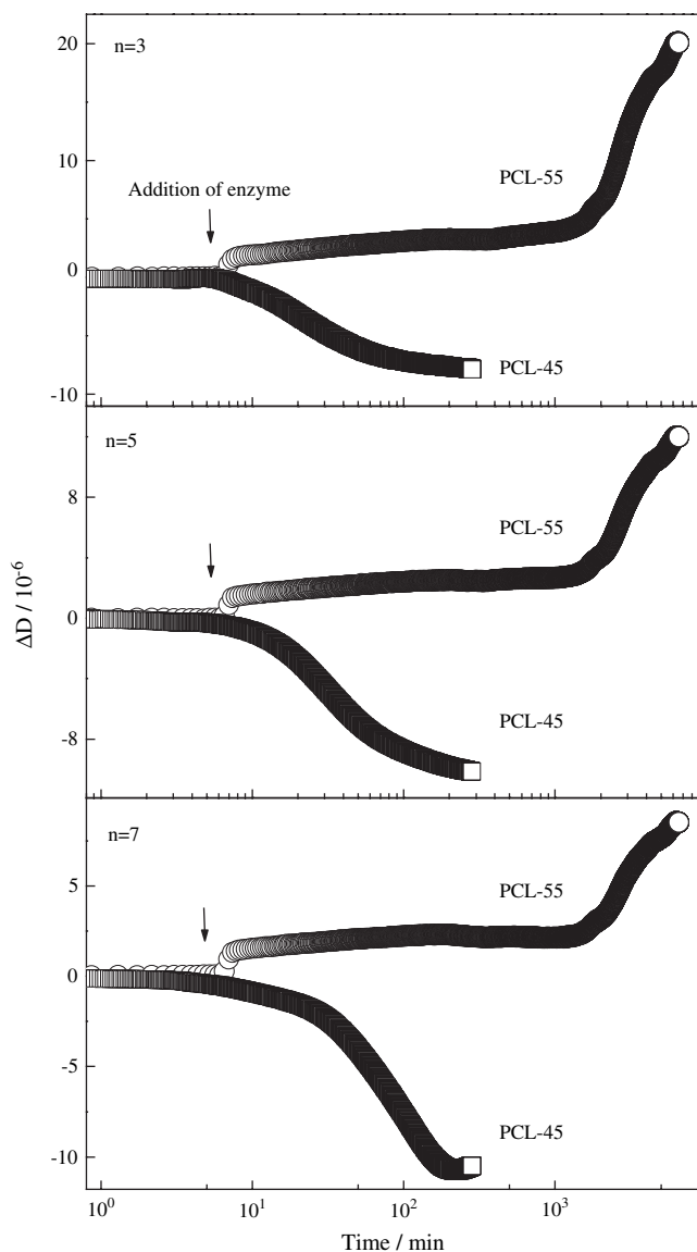
Fig. 3. The dissipation shift ( \Delta D ) of QCM during enzymatic degradation of PCL-45 and PCL-55 catalyzed by lipase PS, where C_e = 0.5 mg/mL and n = 3, 5, 7 .
