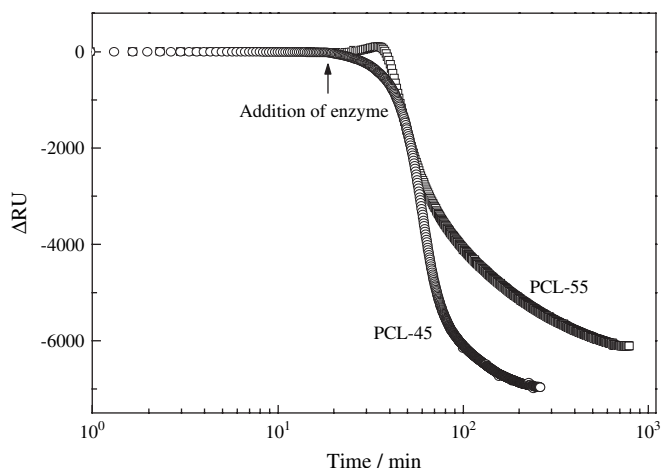
Fig. 5. The signal response shift ( \Delta RU ) of SPR for PCL-45 and PCL-55 after lipase PS was introduced, where C_e = 0.5 mg/mL.
