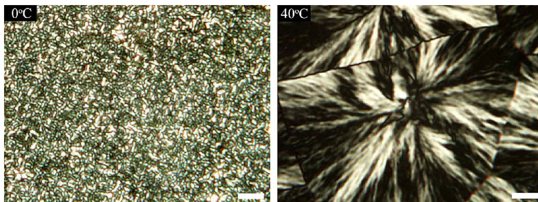
Fig. 1. The polarized optical micrographs of PCL spherulites after melt-crystallizing at 0 °C and 40 °C. The scale bar is 10 µm.
