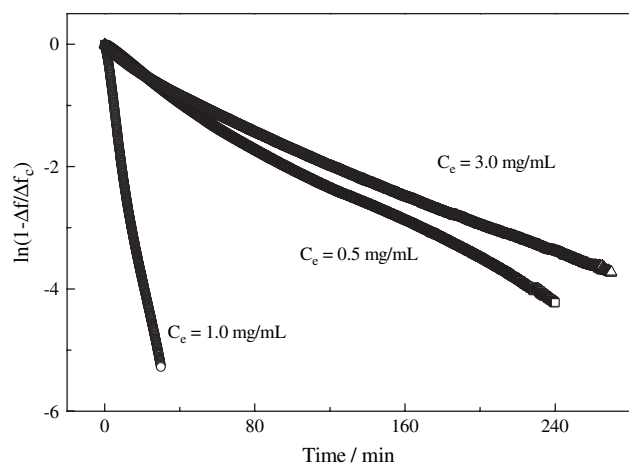
Fig. 6. Time dependence of \ln(1 - \Delta f/\Delta f_c) for the enzymatic degradation of PCL-45 film at n = 3 .
