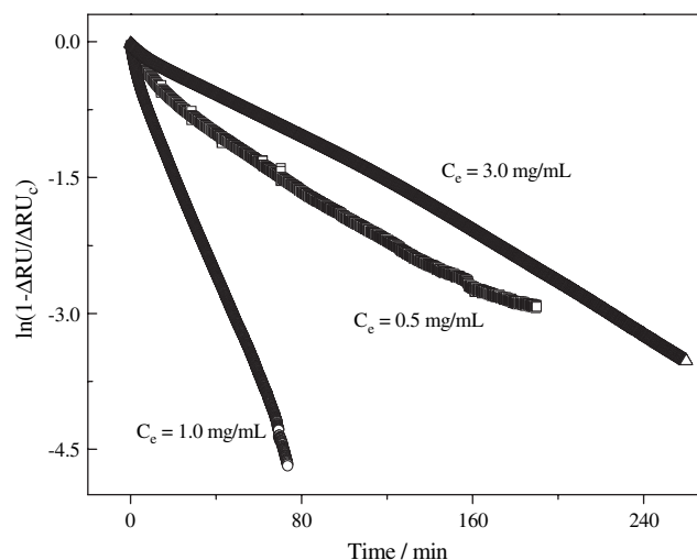
Fig. 7. Time dependence of \ln(1 - \Delta RU/\Delta RU_c) for the enzymatic degradation of PCL-45 film.
