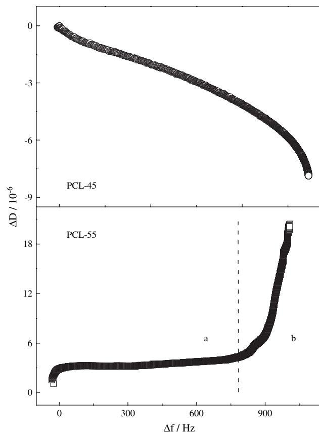
Fig. 4. The relations of \Delta D vs \Delta f for enzymatic degradation of PCL-45 and PCL-55 catalyzed by lipase PS at n = 3 , where C_e = 0.5 mg/mL.
